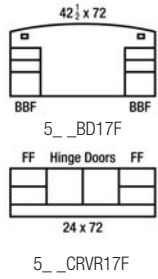
"U" Workstation - Left
