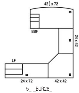
"L" Workstation - Right
