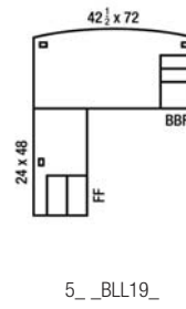
"U" Workstation - Left
