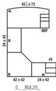
Bow Front Desk
